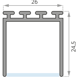
LIPOD 26×24,5 mm
